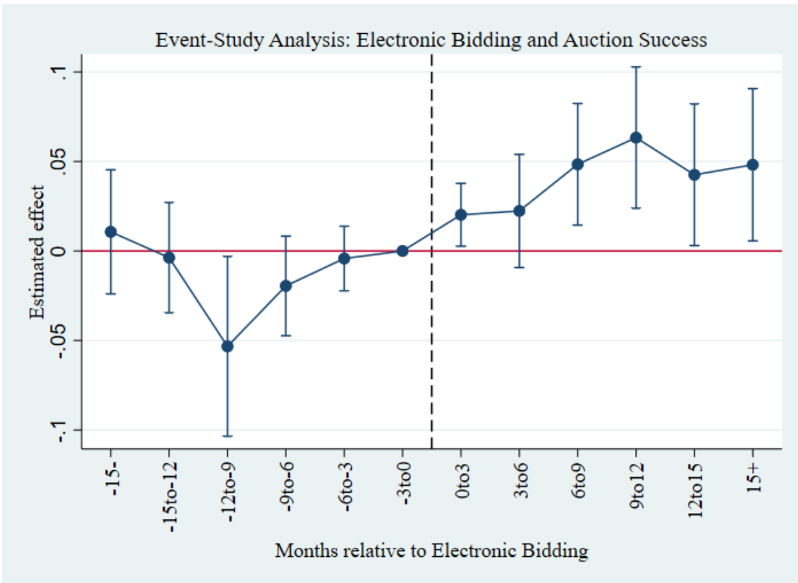
Figure 3: Event study estimates of electronic bidding on foreclosure auction success.
