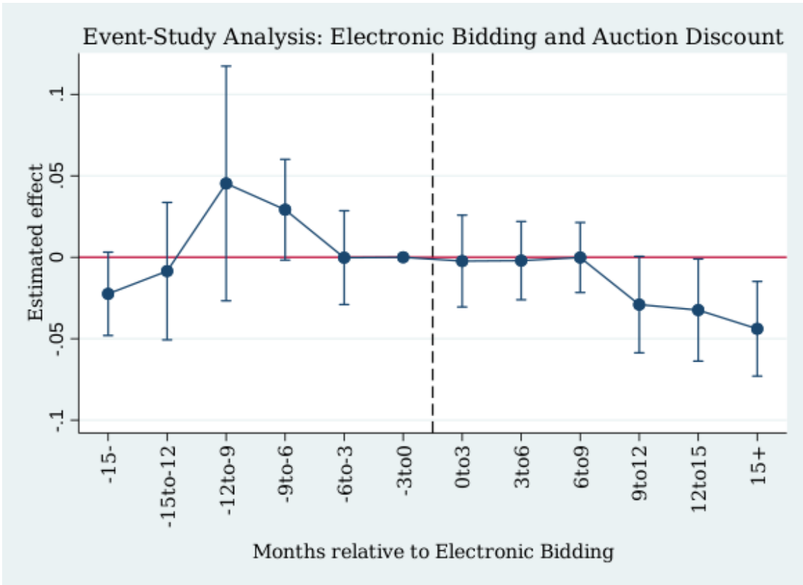
Figure 5: Event study estimates of electronic bidding on foreclosure auction discount.
